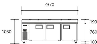
Integral front elevation
