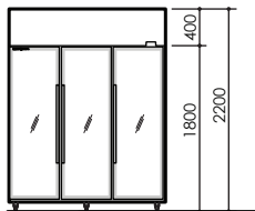
Integral front elevation
