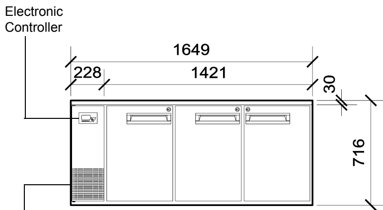
Evaporator box and service compartment
